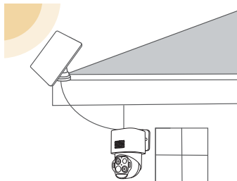
Wall Mounting
